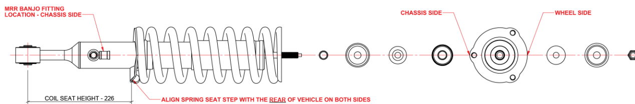
TOYOTA HILUX (2005-ON) RIGHT HAND STRUT SHOWN
