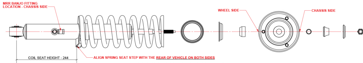
MITSUBISHI PAJERO (2000-ON) RIGHT HAND STRUT SHOWN
