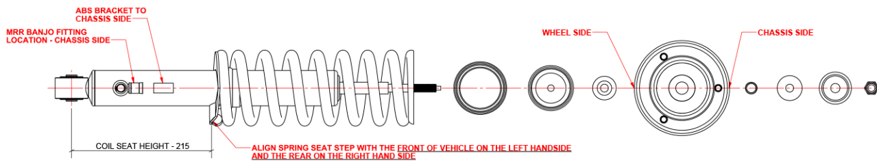
MITSUBISHI TRITON (MQ-MR) RIGHT HAND STRUT SHOWN
